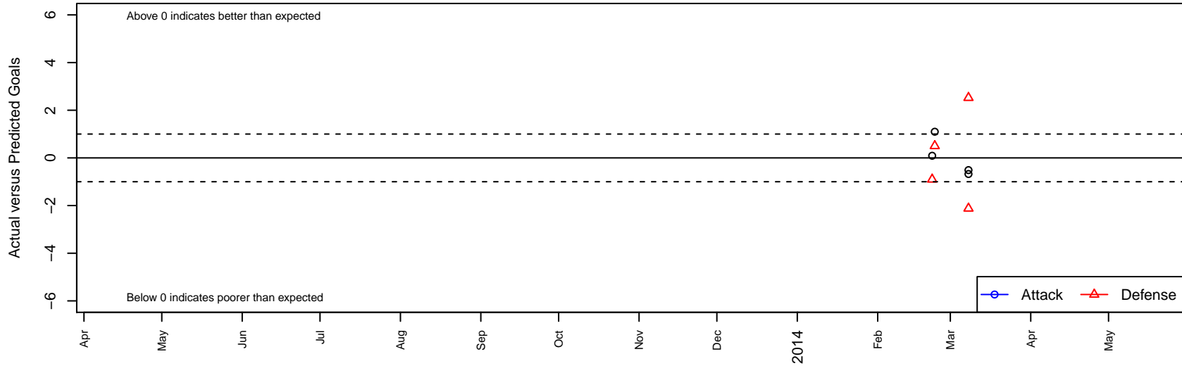
Quest SC White B00 Dots are actual minus expected GF (blue circles) and GA (red triangles). Blue line is smoothed change in attack strength. Red is smoothed change in defense strength.
